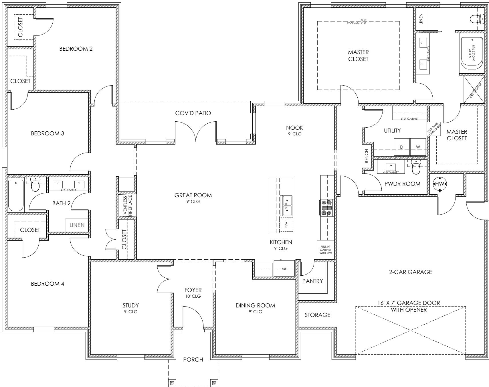
2545_4BD2F2HBA71_2C 2,545 SF LIVING AREA SCALE: 1/8"=1'-0" AT 8.5" X 11"
